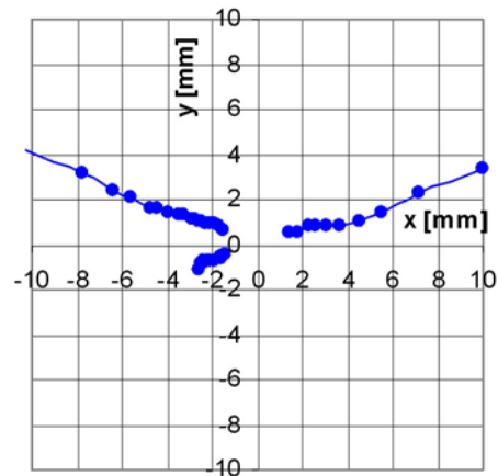
Fig. 9. Crack propagation in specimen No. 13
